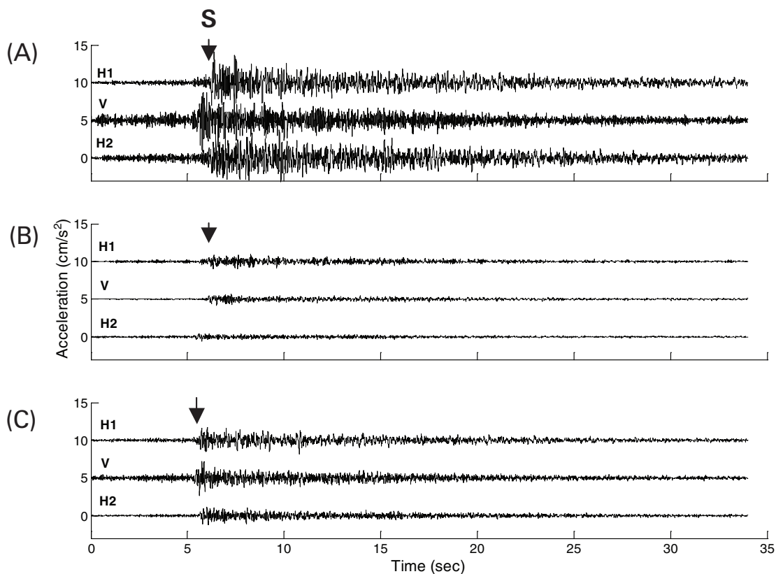
▲ Figure 5. Acceleration recordings from the June 2, 2005, Ridgely, Tennessee, earthquake at vertical strong-motion array VSAS. (A) surface, (B) 30 m deep, (C) 260 m deep.
